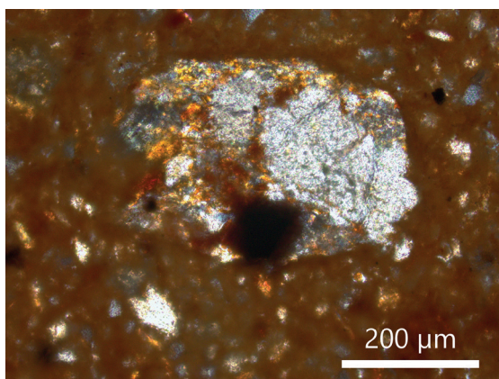
Fig. 14. Sample P4 – schist fragment (CPL); photo by J. Michniewicz.
