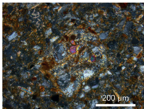
Fig. 15. Sample P11 – plagioclase-biotite-epidote metashale fragment (photo by J. Michniewicz).
